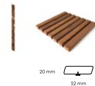
Rhombus (QuickClip®)
